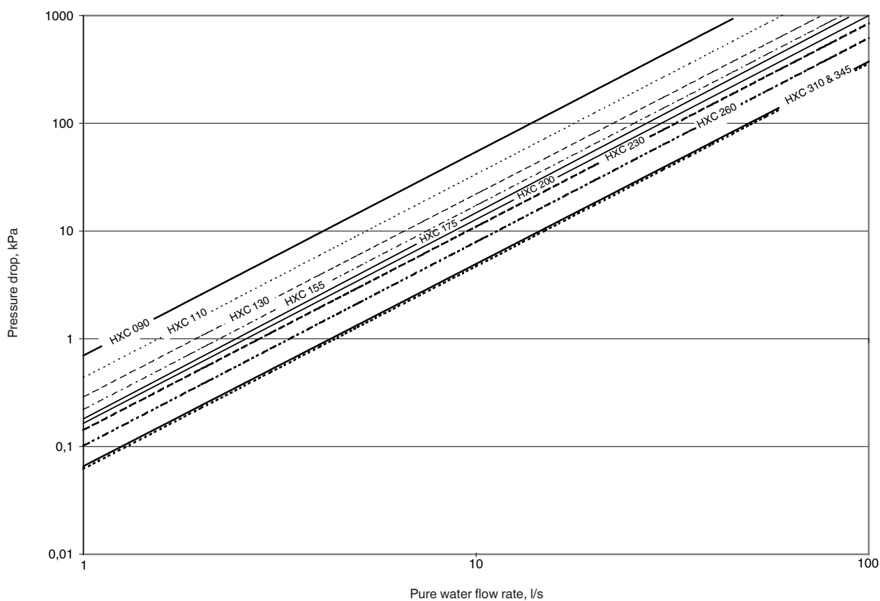
Cooler pressure drop, 30HXC low-brine version
