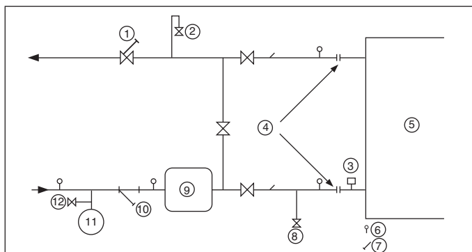
Typical water circuit diagram
